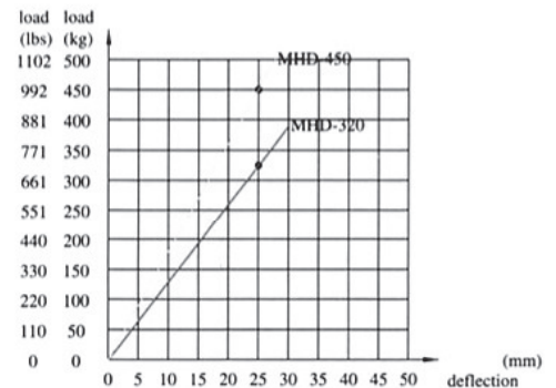
LOAD DEFLECTION CURVE/POINT MEANS THE BEST DEFLECTION
